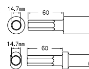
Hex. Shank
