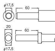
Round Shank
